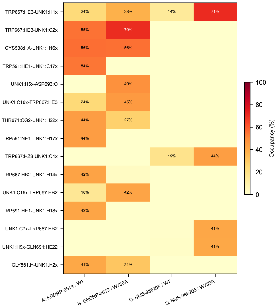
H-bond occupancy — top 15 across all cases
